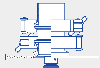
Tri-Clamp connection
